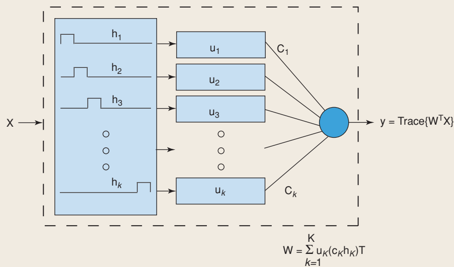
[FIG4] Hierarchical discriminant component analysis. EEG signatures of target detection events are estimated using multiple linear discriminators each trained at a different time window relative to the image onset. A set of k = 1 \dots K nonoverlapping windows functions h_k are chosen and the discriminators u_k each associated with the corresponding time window are trained separately. At a second level, the discriminators u_k are fixed and coefficients c_k are learned. The resulting discriminant model takes the form of (4) where additional structure has been enforced on the temporal weights: v_k = h_k c_k .
